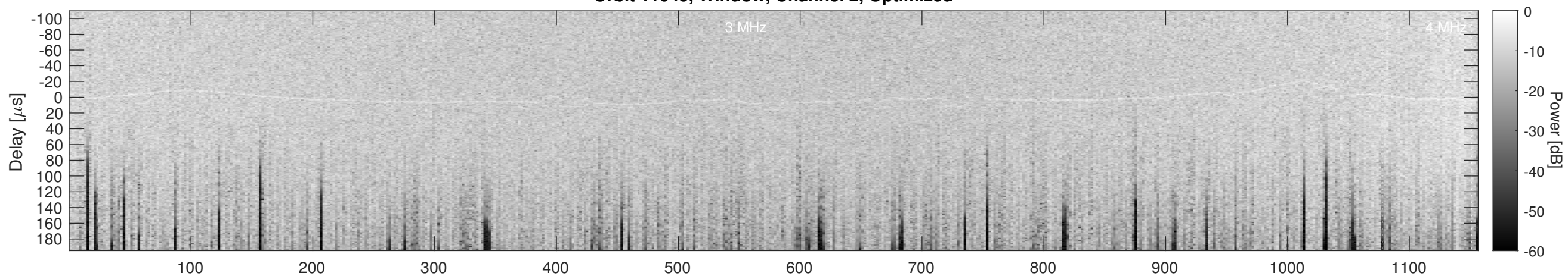
Orbit 11045, Cluttergram
