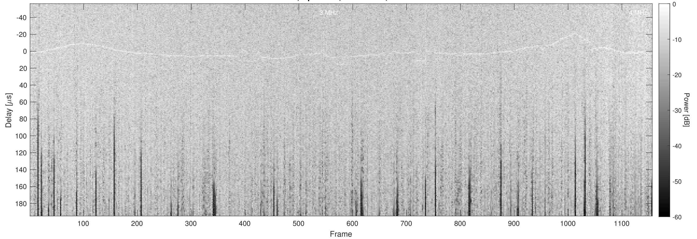
Orbit 11045, Optimized, No Window, Channel 2
