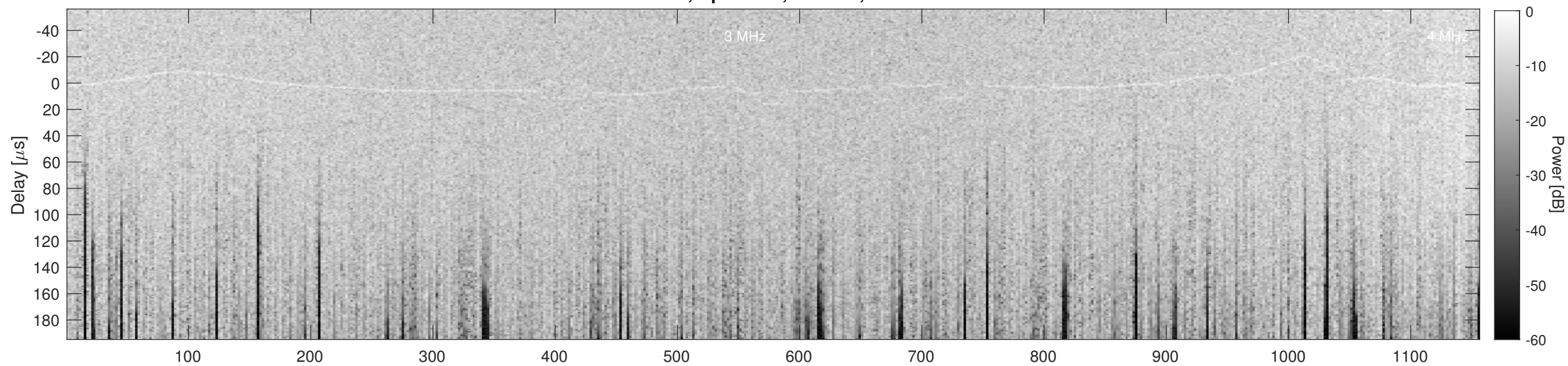
Orbit 11045, Cluttergram
