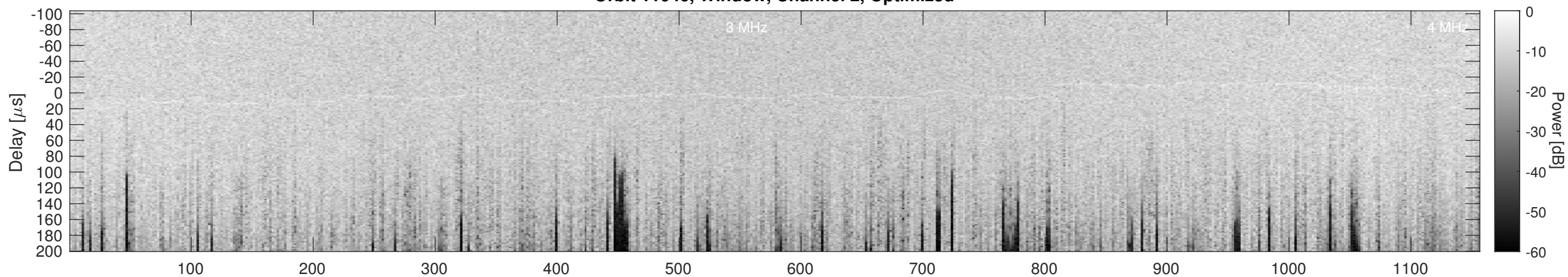
Orbit 11046, Cluttergram
