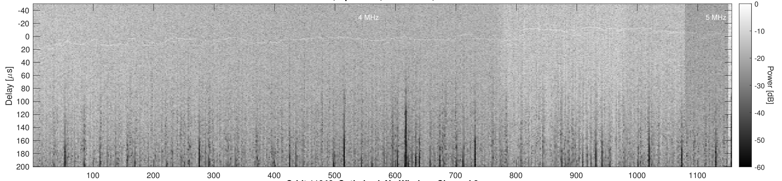
Orbit 11046, Optimized, No Window, Channel 2
