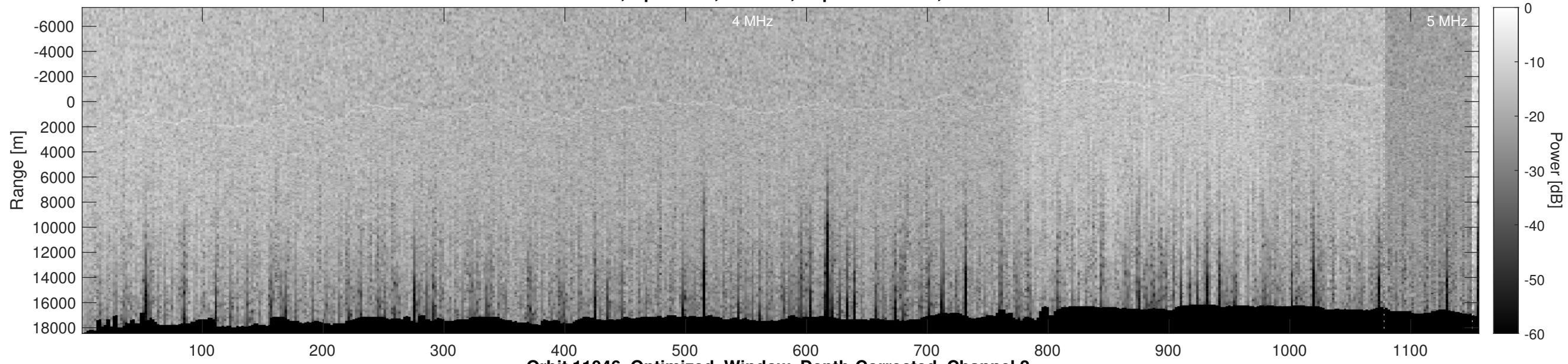
Orbit 11046, Optimized, Window, Depth-Corrected, Channel 2
