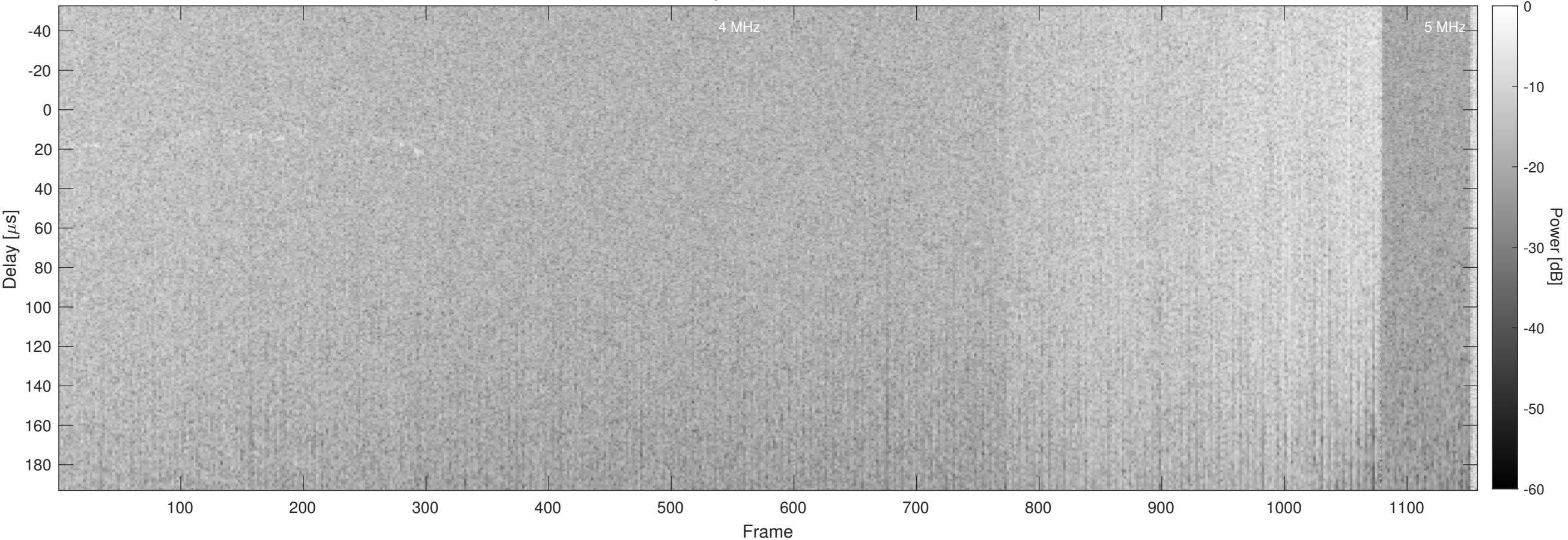
Orbit 11047, Chapman, No Window, Channel 2
