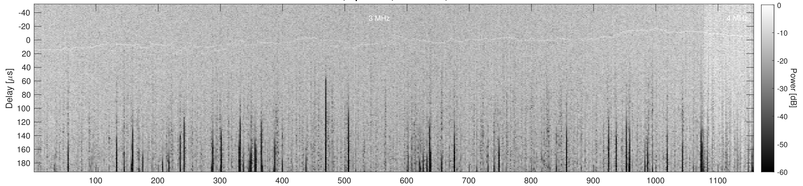
Orbit 11047, Cluttergram
