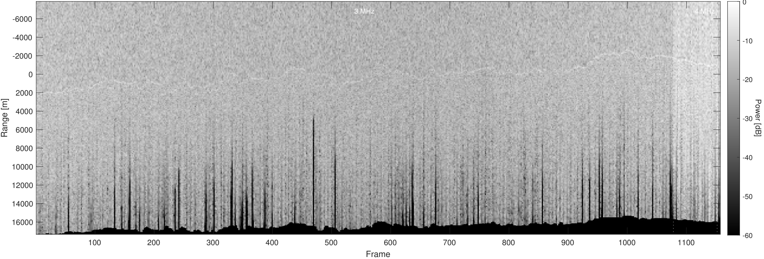
Orbit 11047, Optimized, Window, Depth-Corrected, Channel 2
