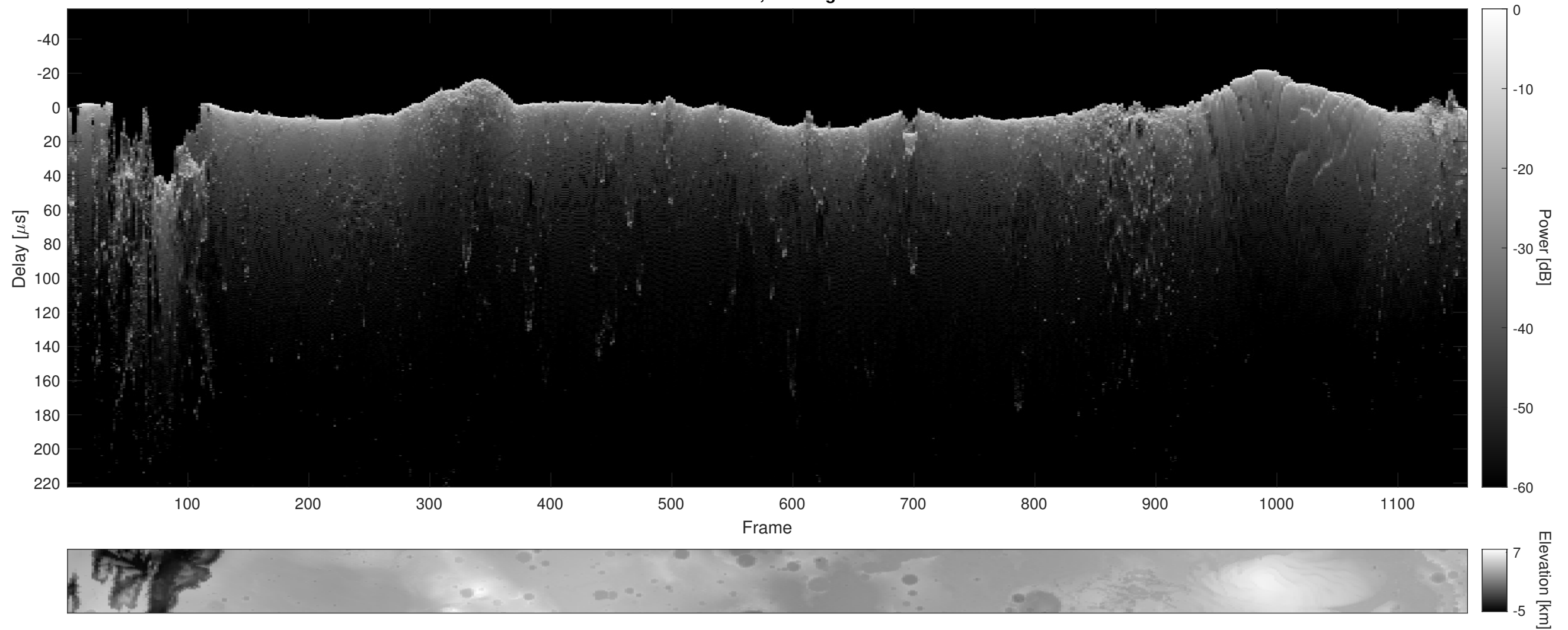
Orbit 11048, Cluttergram
