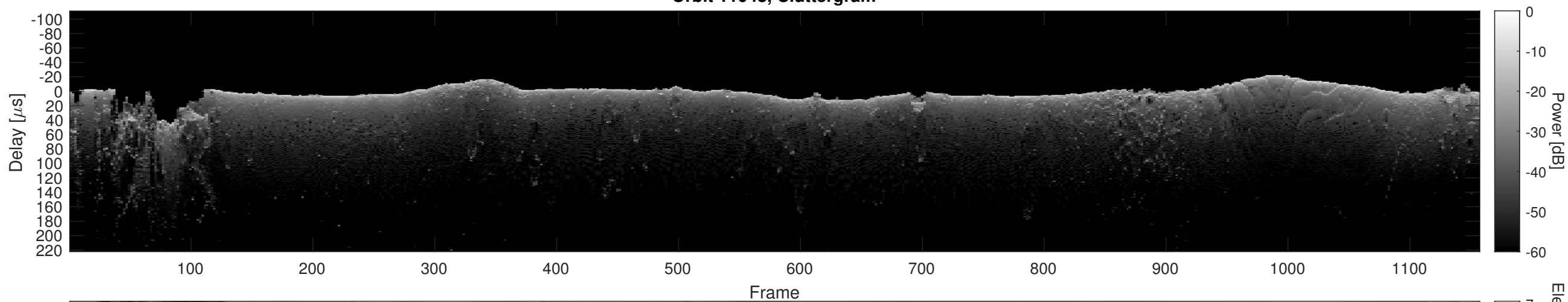
Orbit 11048, Cluttergram
