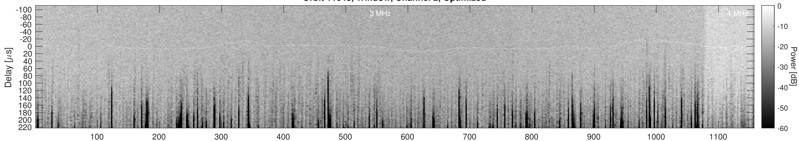
Orbit 11048, Cluttergram
