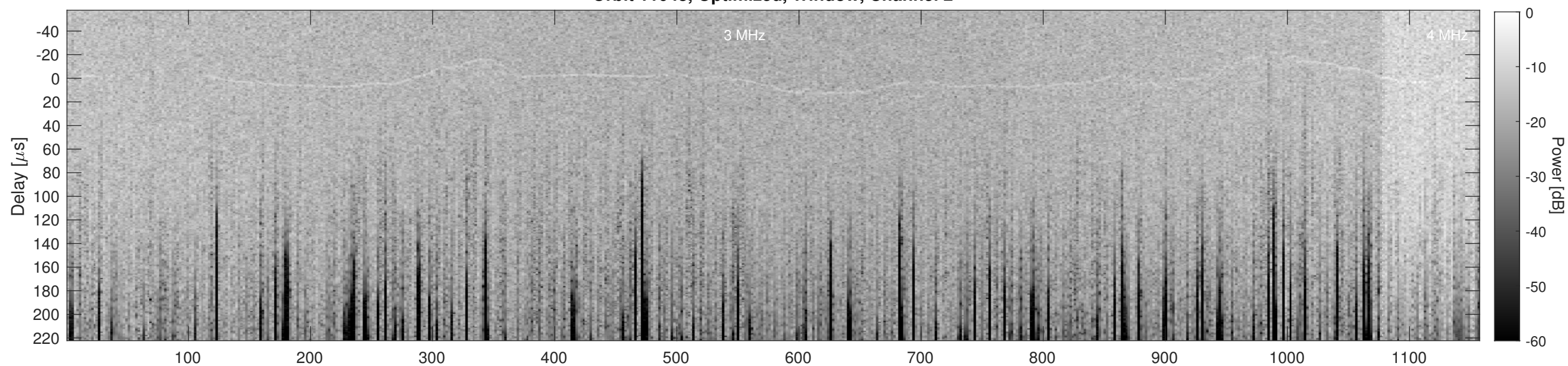
Orbit 11048, Cluttergram
