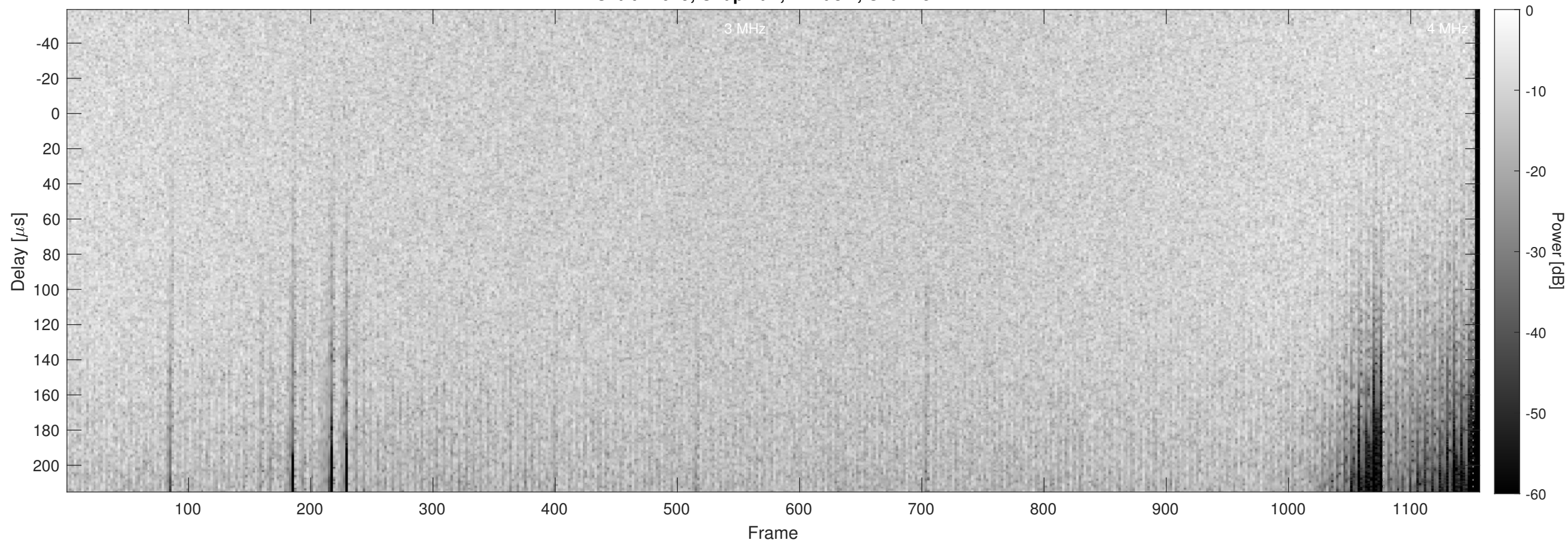
Orbit 11049, Chapman, Window, Channel 2
