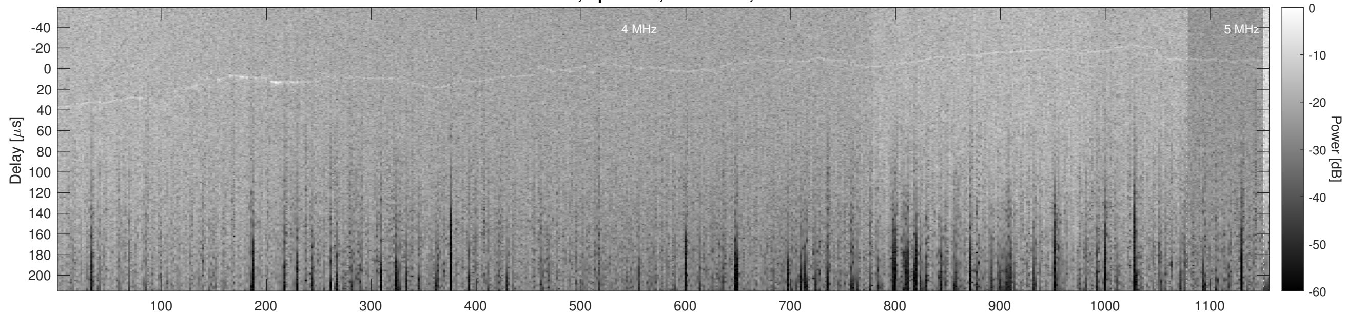
Orbit 11049, Optimized, No Window, Channel 2
