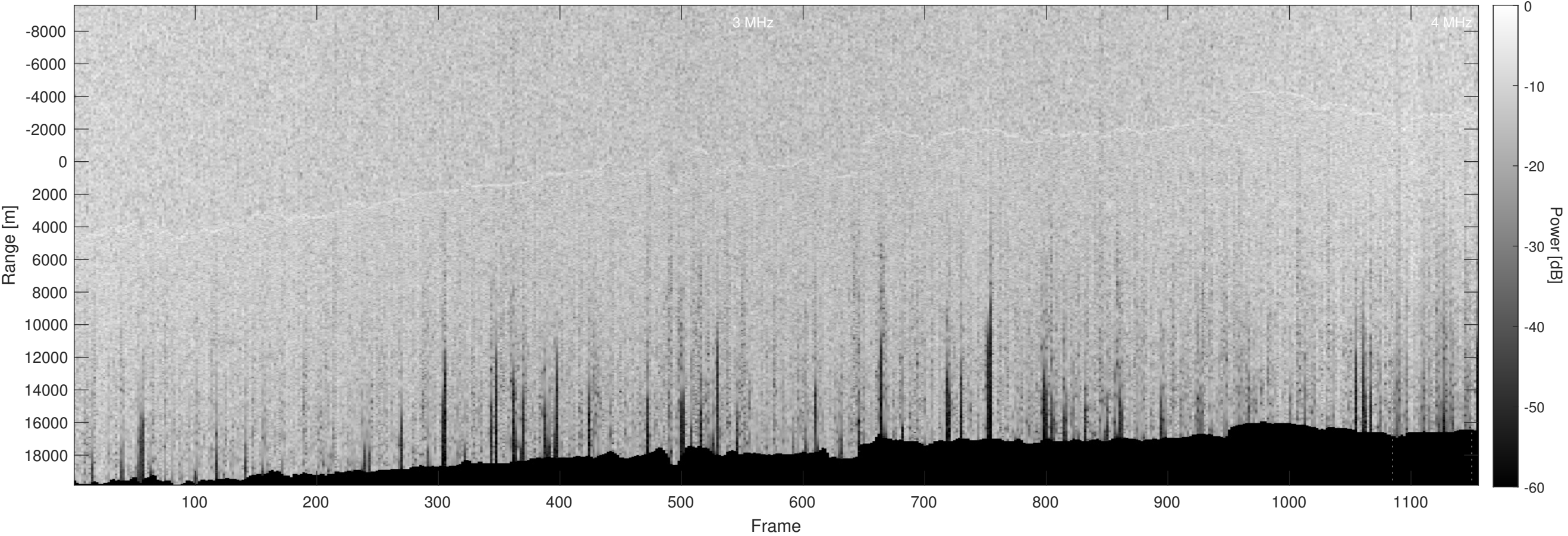
Orbit 11051, Optimized, No Window, Depth-Corrected, Channel 2
