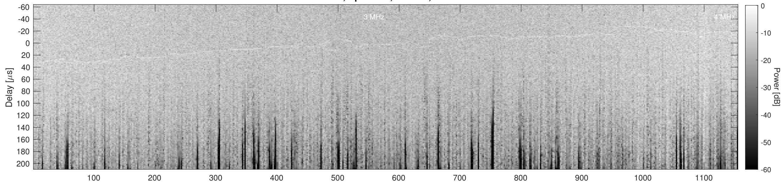
Orbit 11051, Cluttergram
