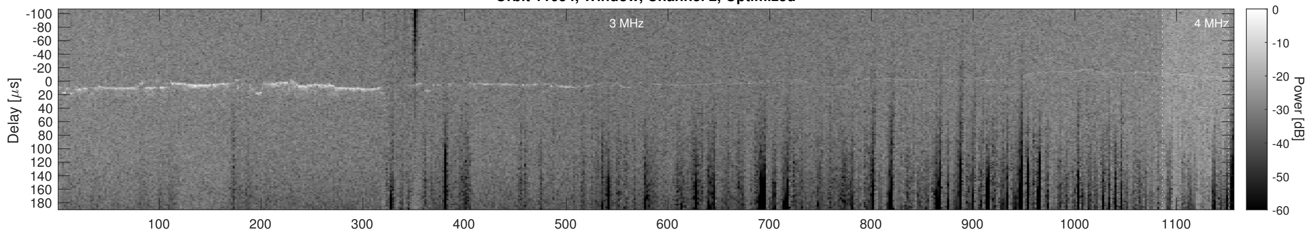
Orbit 11054, Cluttergram
