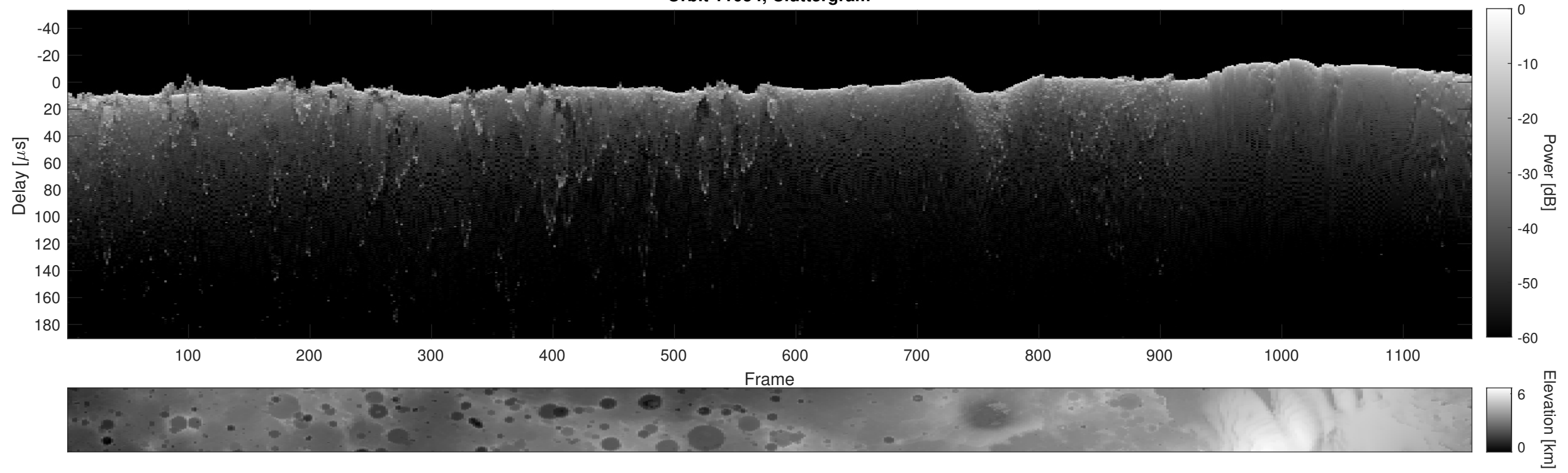
Orbit 11054, Cluttergram
