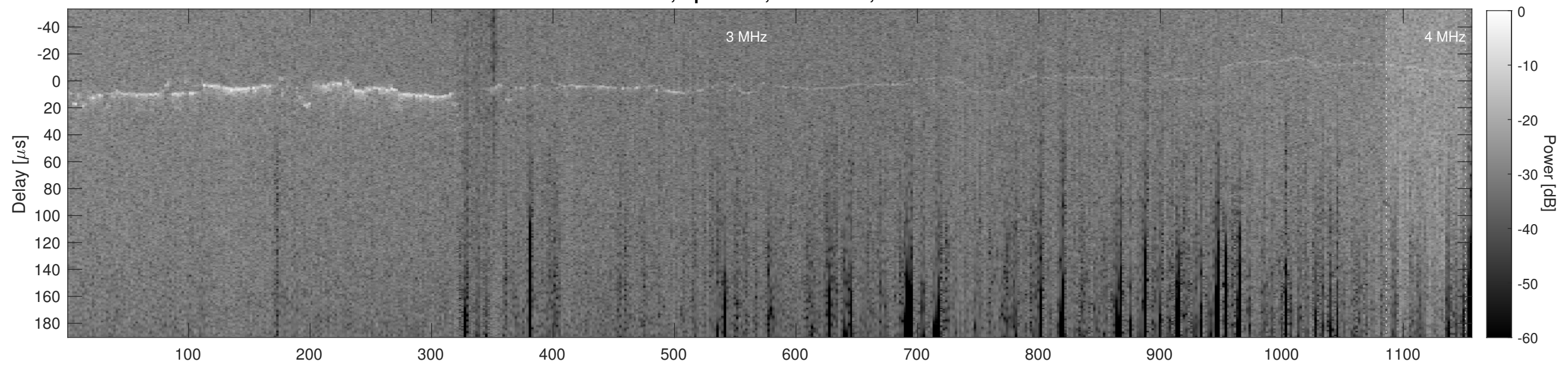
Orbit 11054, Cluttergram
