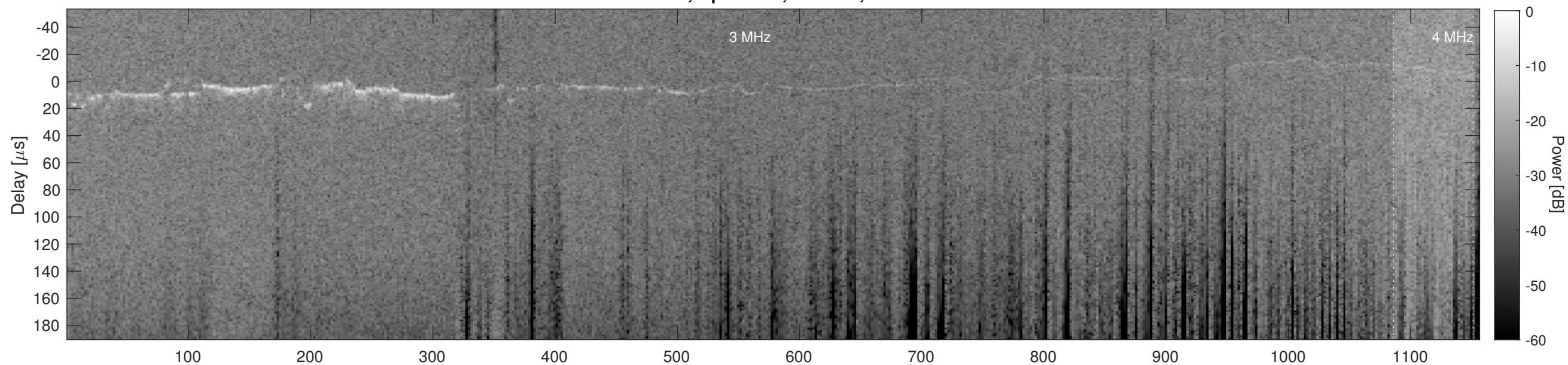
Orbit 11054, Cluttergram
