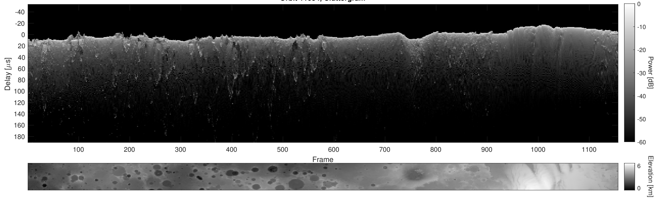
Orbit 11054, Cluttergram
