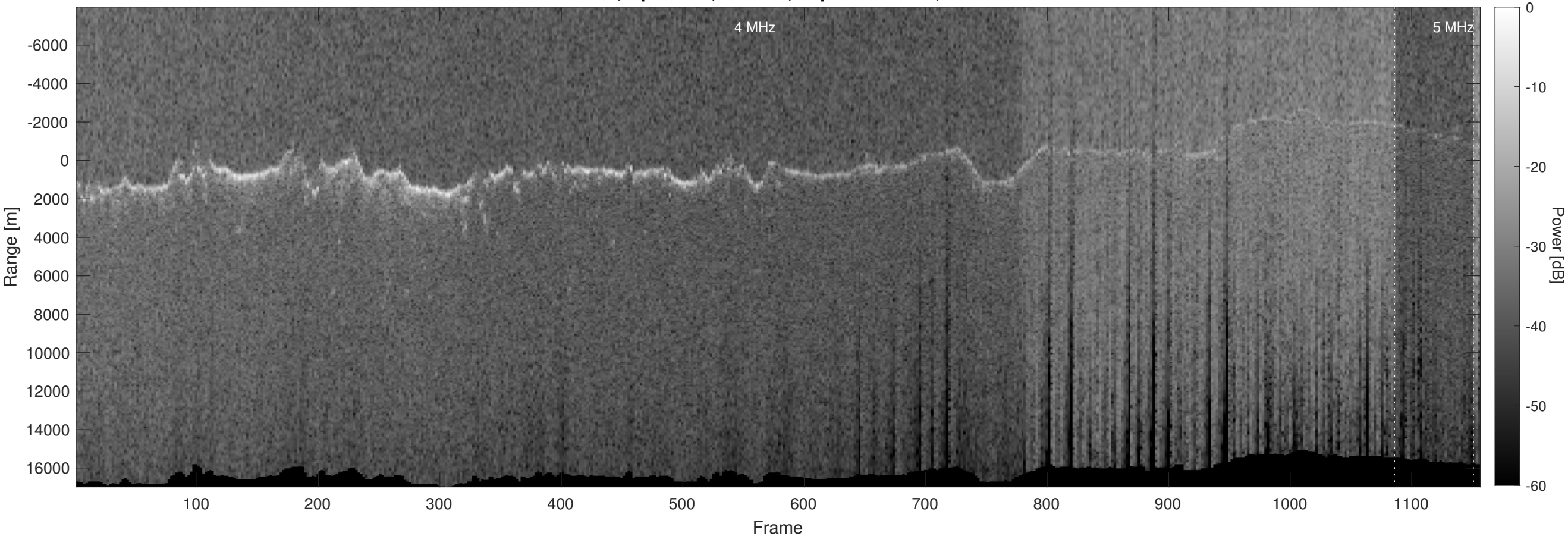
Orbit 11054, Optimized, Window, Depth-Corrected, Channel 2
