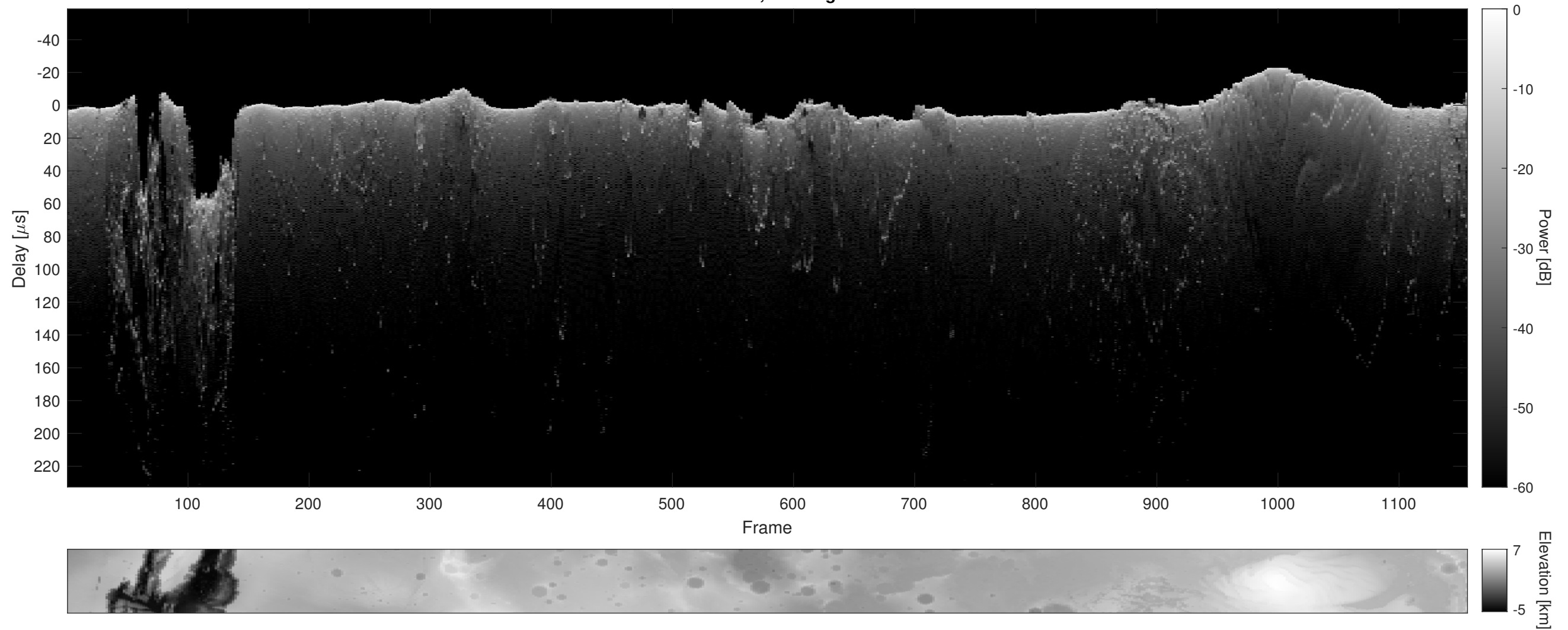
Orbit 11055, Cluttergram
