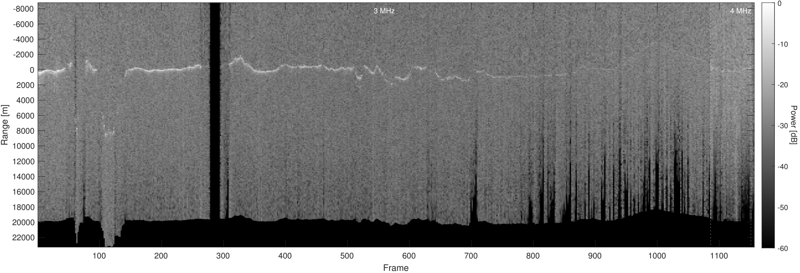
Orbit 11055, Optimized, No Window, Depth-Corrected, Channel 2
