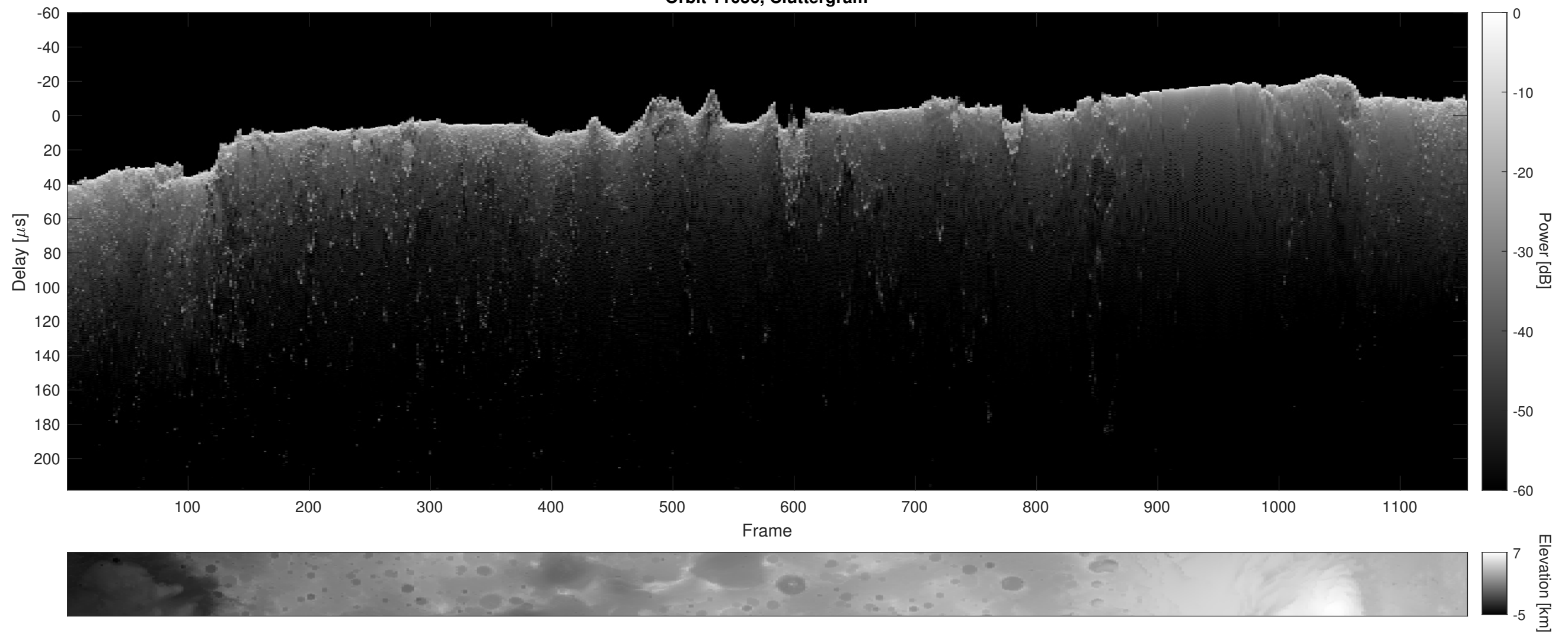
Orbit 11056, Cluttergram
