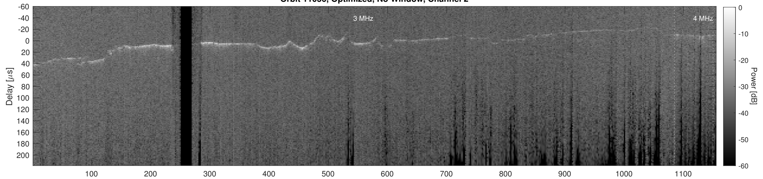
Orbit 11056, Cluttergram
