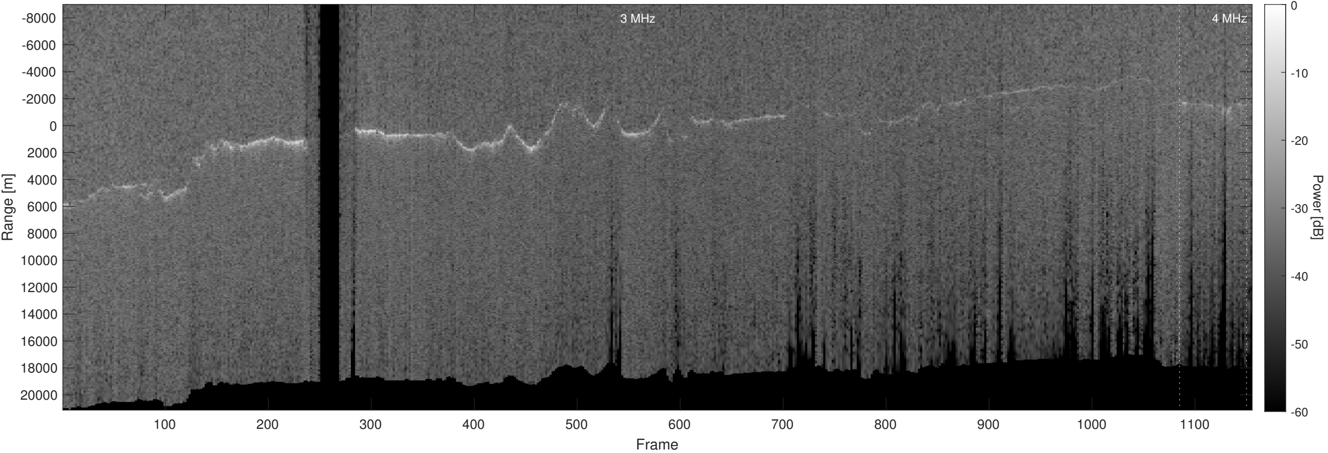
Orbit 11056, Optimized, No Window, Depth-Corrected, Channel 2
