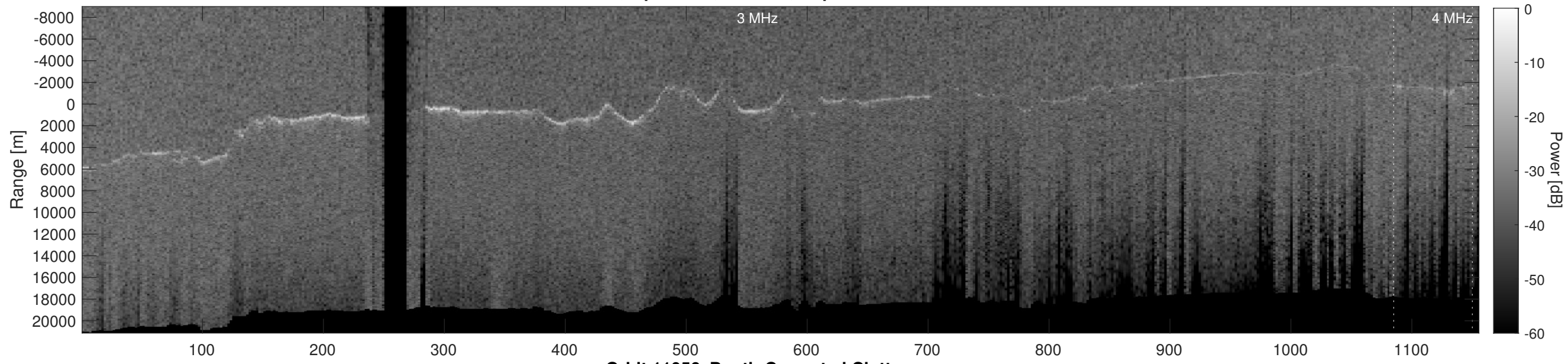
Orbit 11056, Depth-Corrected Cluttergram
