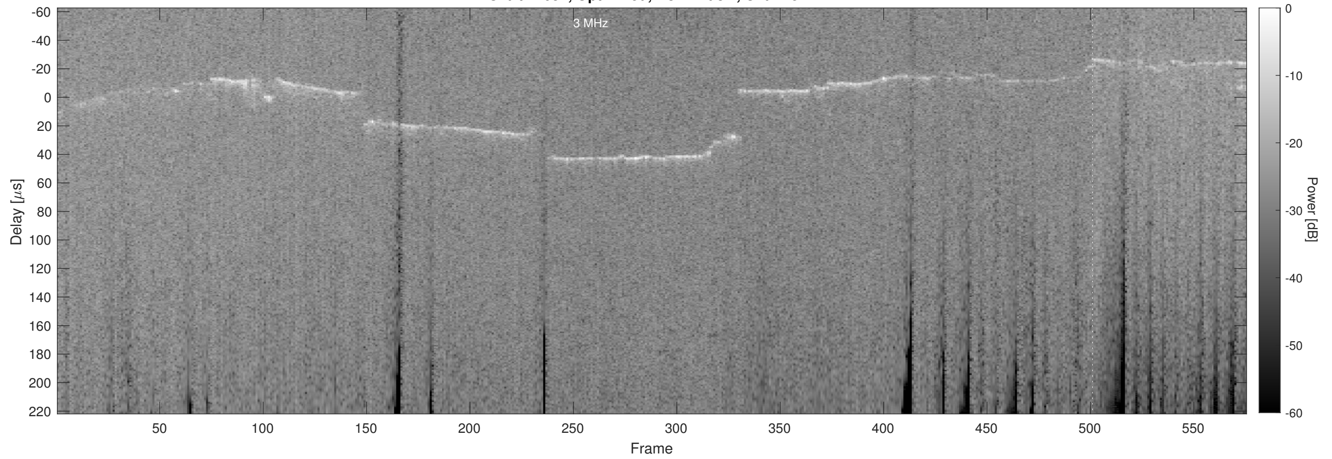
Orbit 11057, Optimized, No Window, Channel 2
