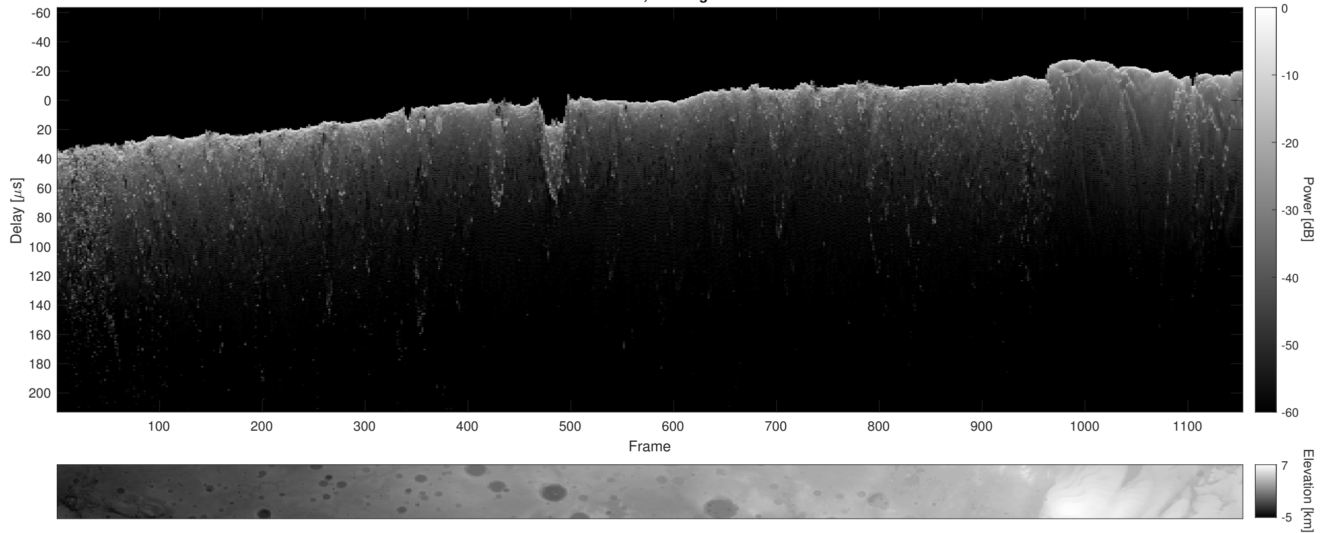
Orbit 11058, Cluttergram
