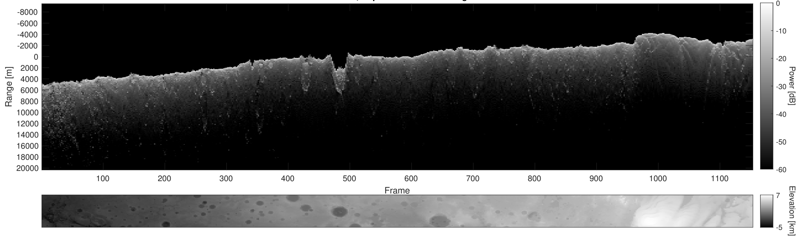
Orbit 11058, Depth-Corrected Cluttergram
