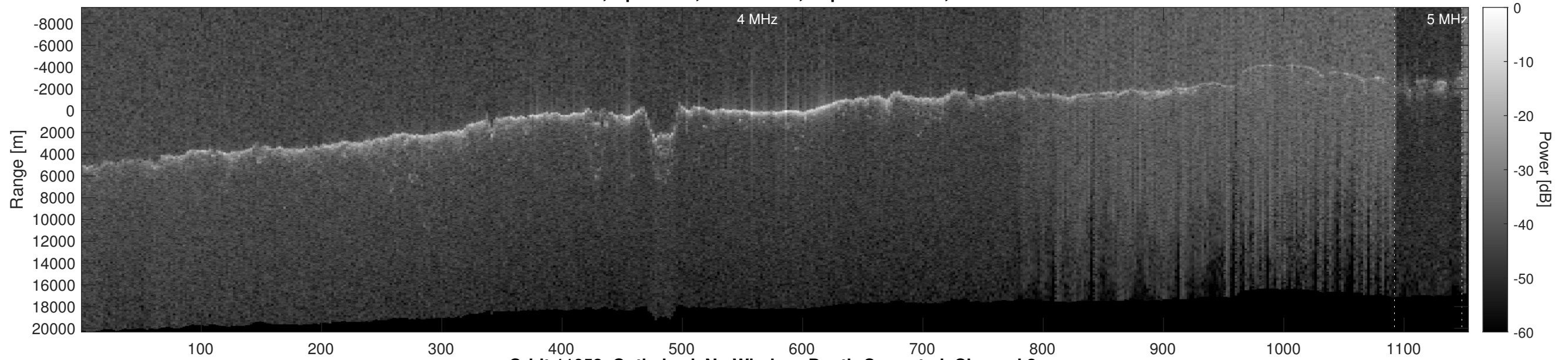
Orbit 11058, Optimized, No Window, Depth-Corrected, Channel 2
