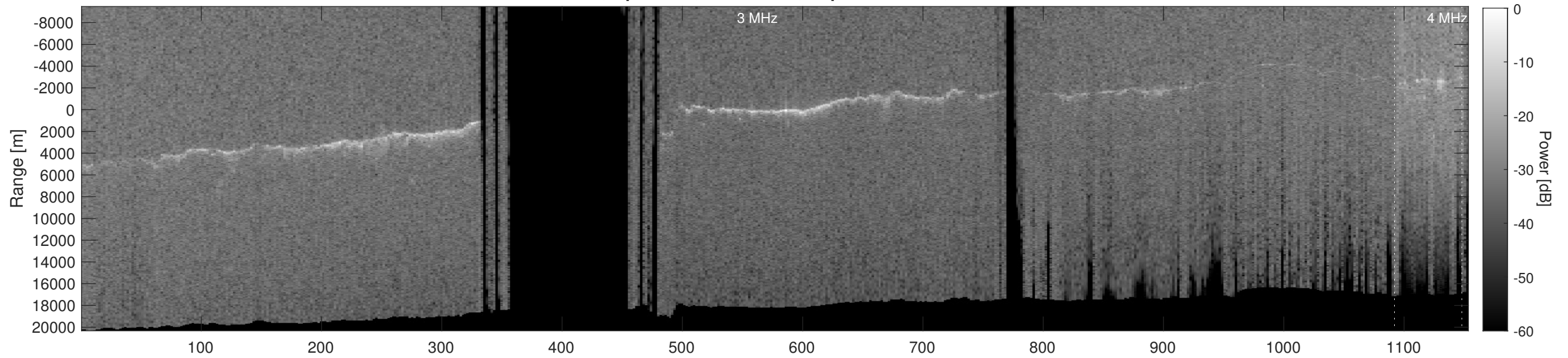
Orbit 11058, Depth-Corrected Cluttergram
