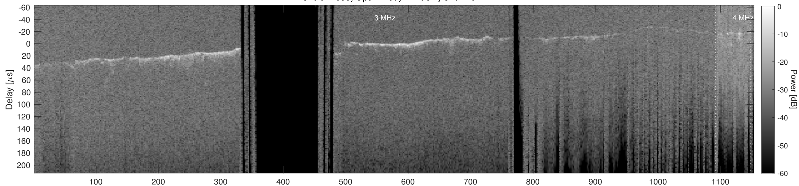
Orbit 11058, Cluttergram
