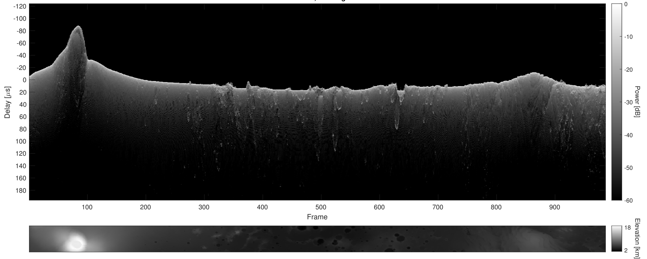
Orbit 11059, Cluttergram
