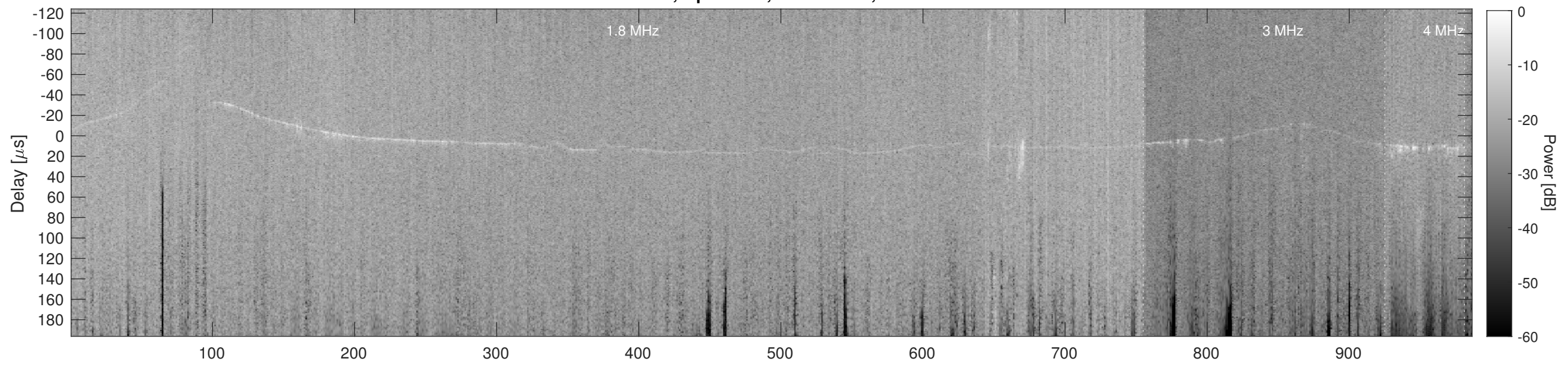
Orbit 11059, Cluttergram
