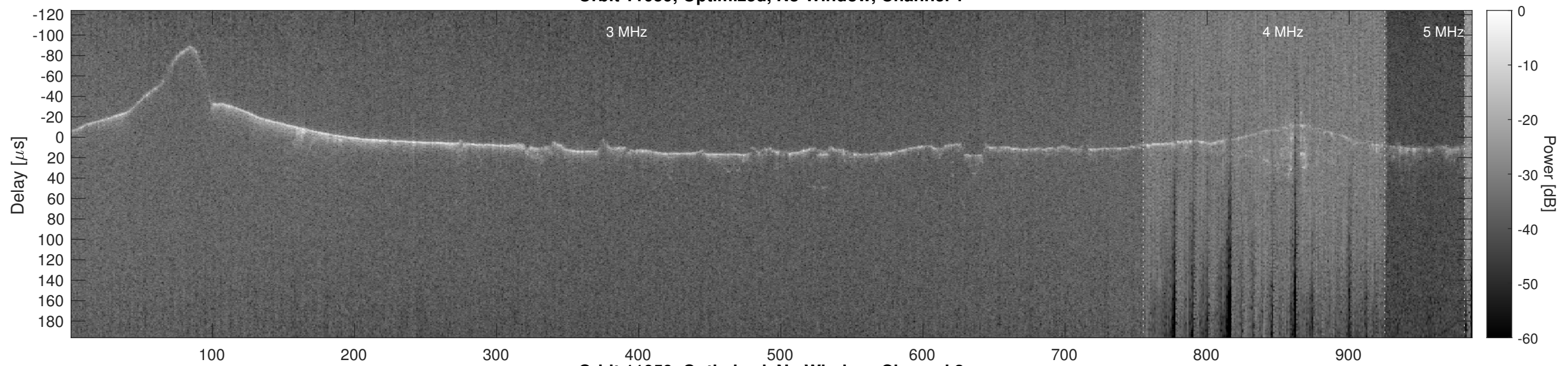
Orbit 11059, Optimized, No Window, Channel 2
