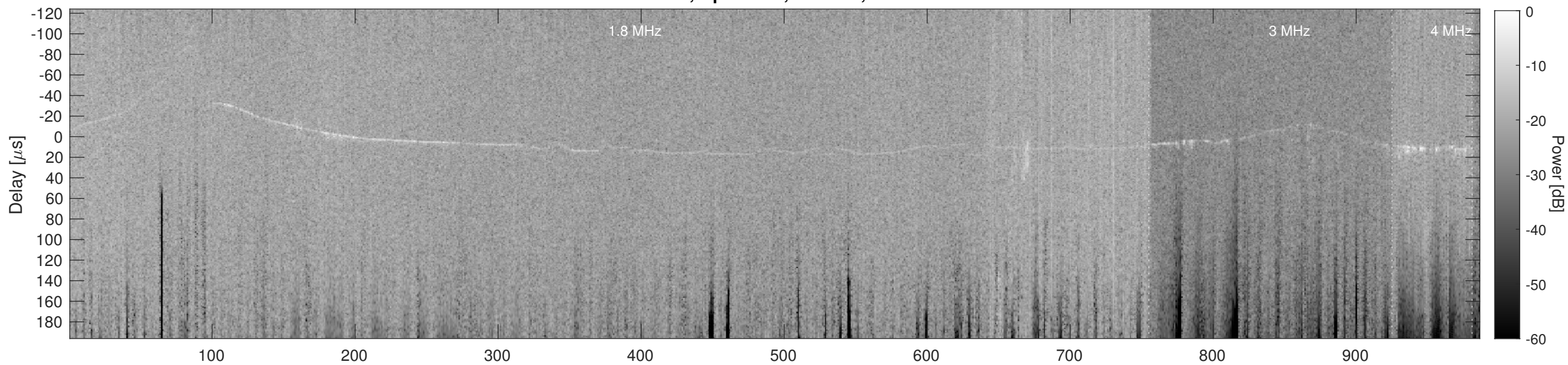
Orbit 11059, Cluttergram
