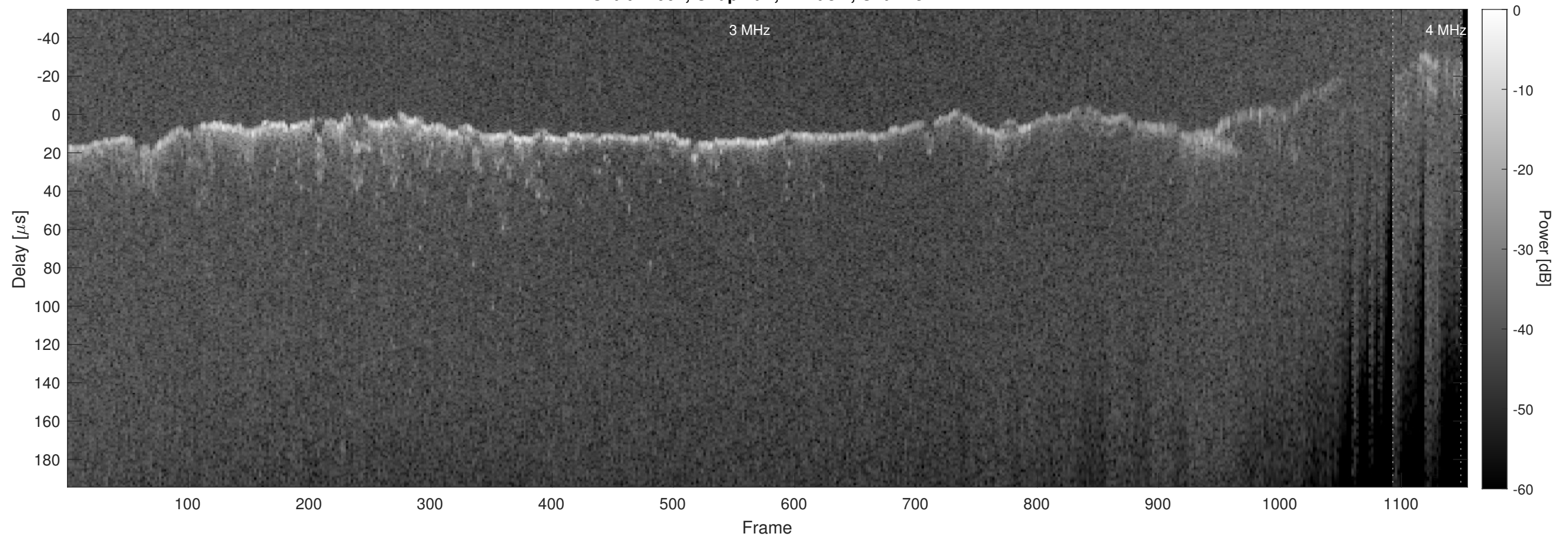
Orbit 11061, Chapman, Window, Channel 2
