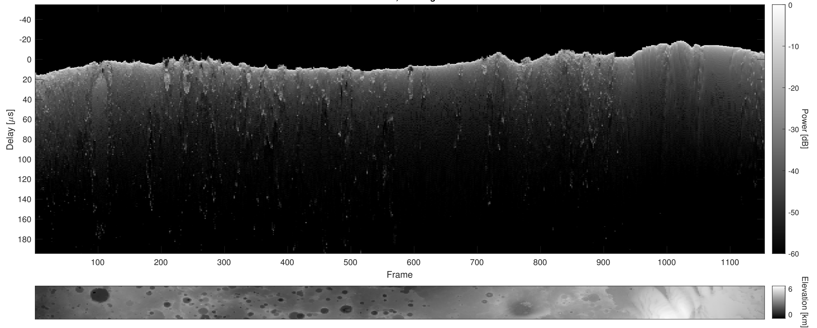
Orbit 11061, Cluttergram
