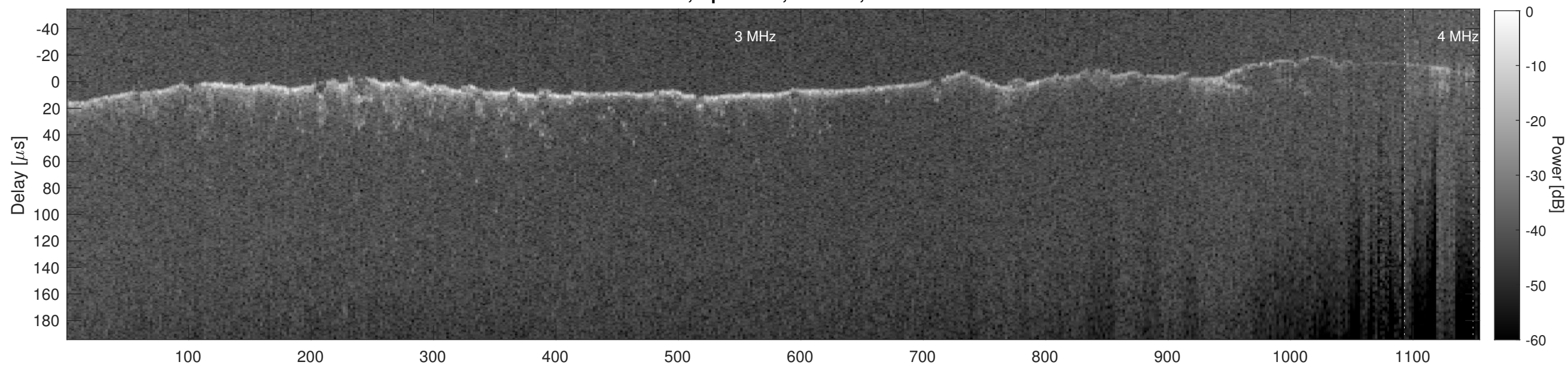
Orbit 11061, Cluttergram
