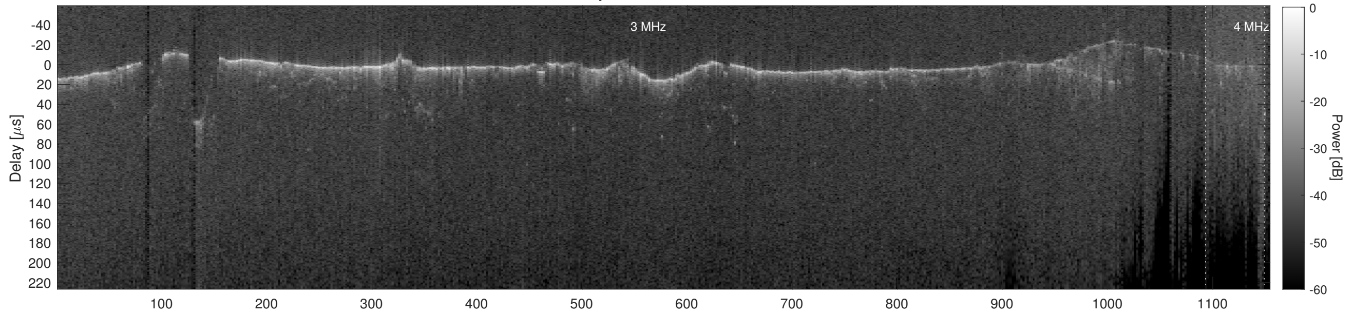
Orbit 11062, Cluttergram
