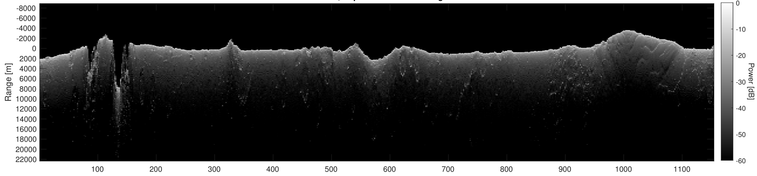
Orbit 11062, Depth-Corrected Cluttergram
