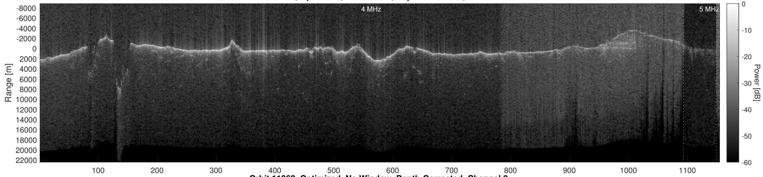
Orbit 11062, Optimized, No Window, Depth-Corrected, Channel 2
