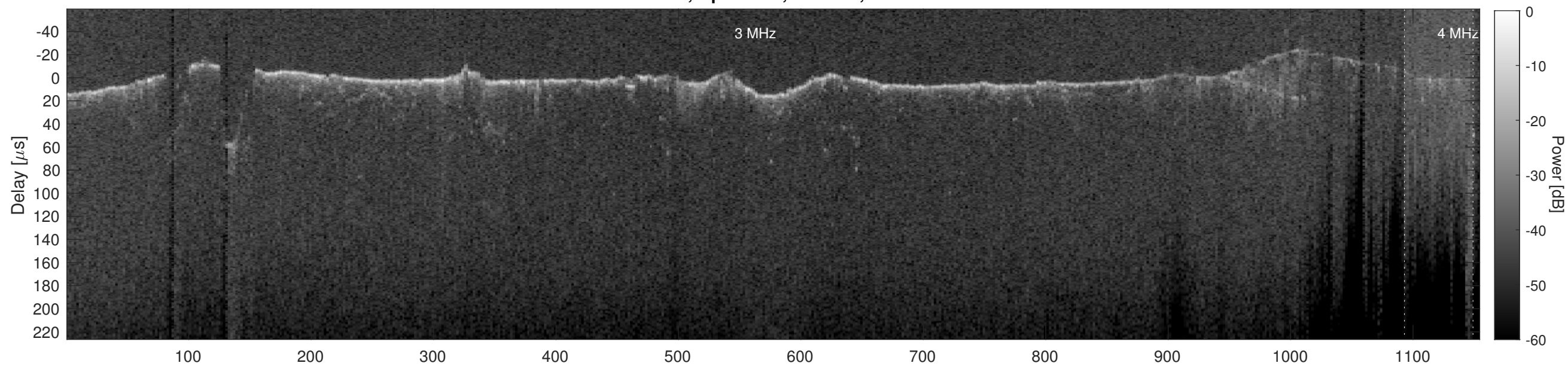
Orbit 11062, Cluttergram
