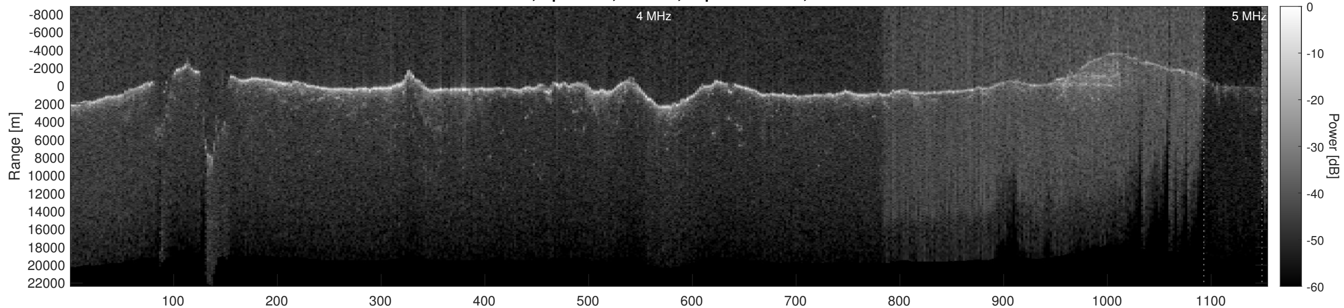
Orbit 11062, Optimized, Window, Depth-Corrected, Channel 2
