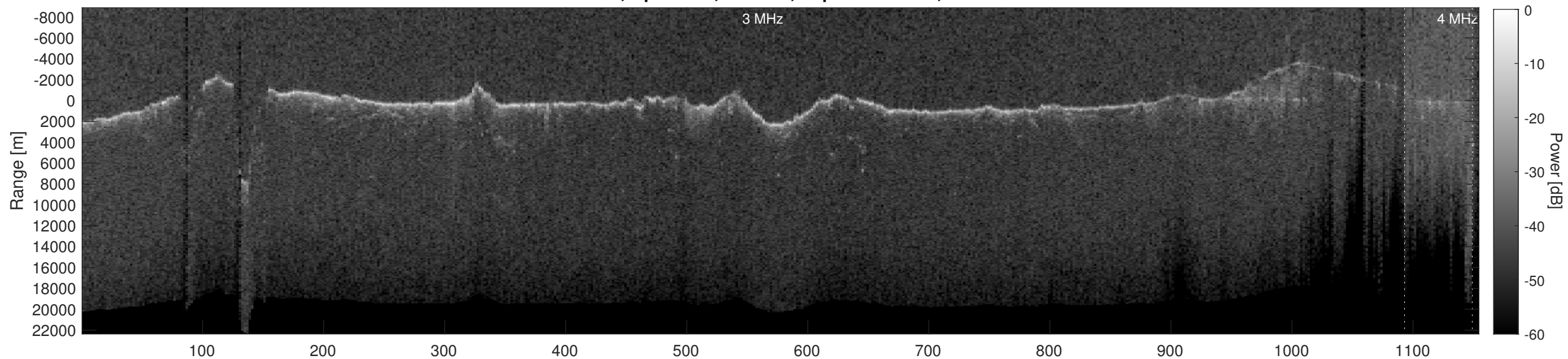
Orbit 11062, Depth-Corrected Cluttergram
