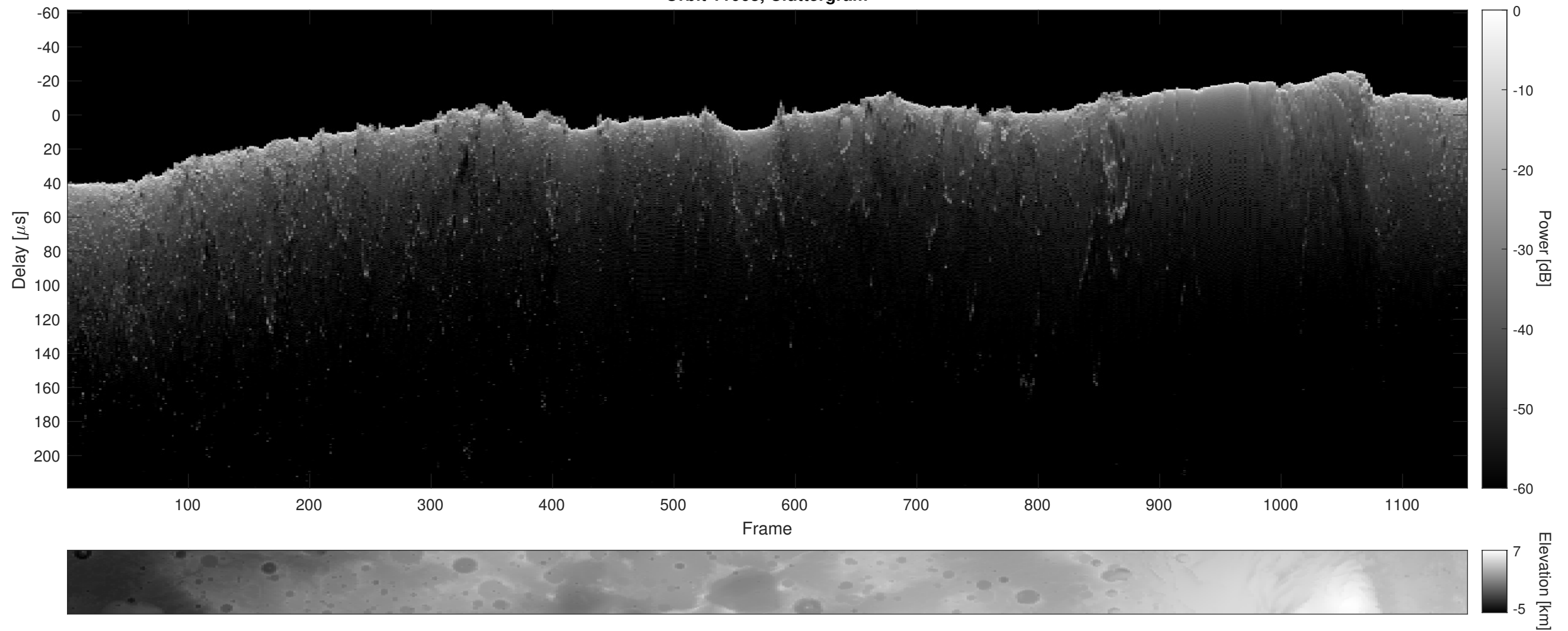
Orbit 11063, Cluttergram
