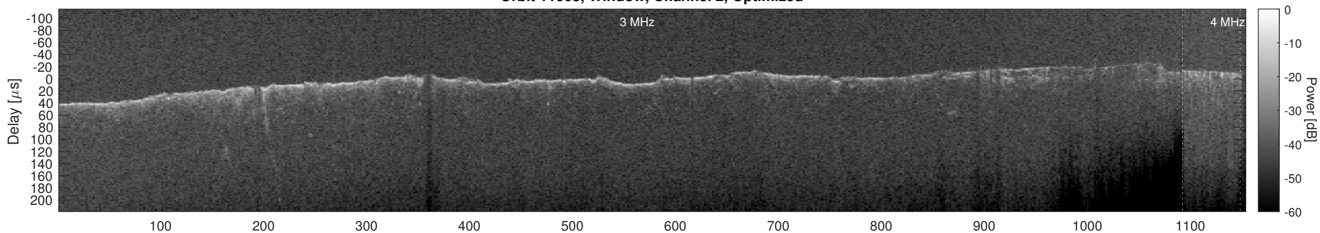
Orbit 11063, Cluttergram
