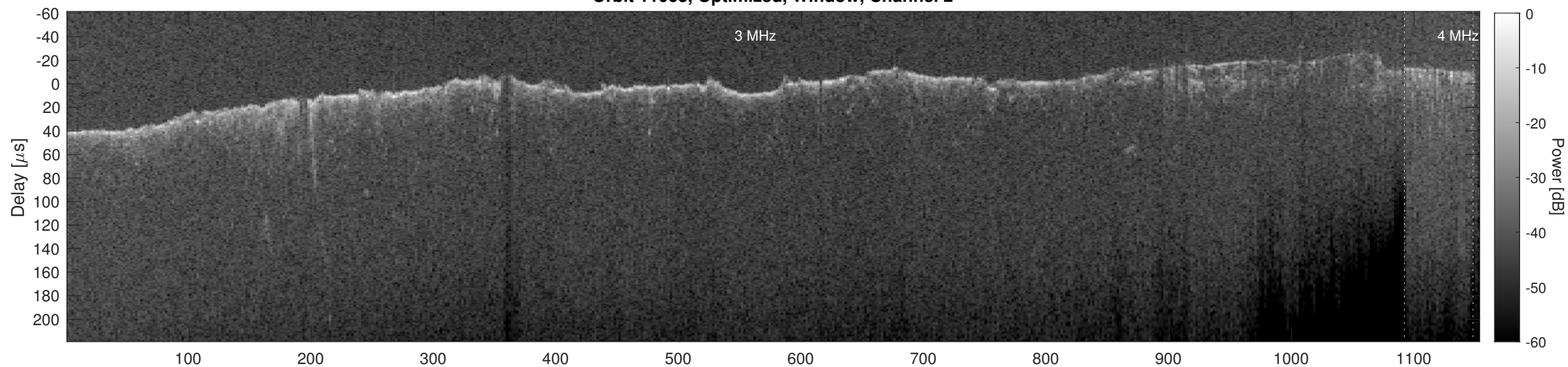
Orbit 11063, Cluttergram
