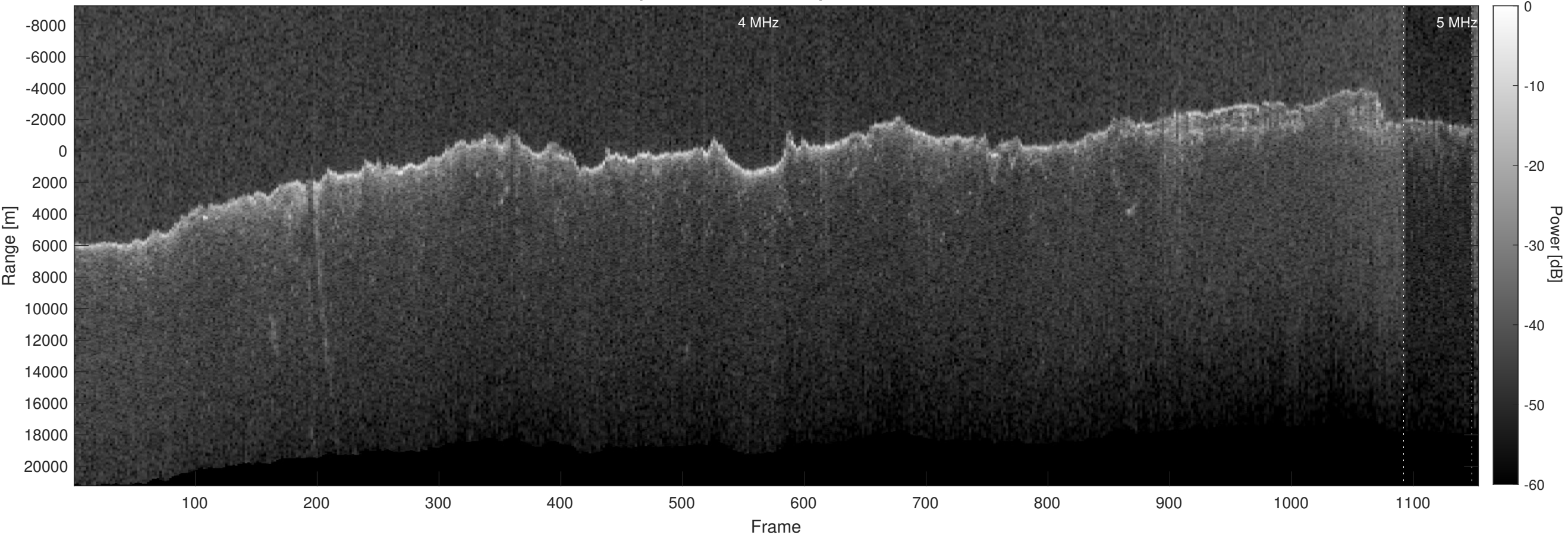
Orbit 11063, Optimized, Window, Depth-Corrected, Channel 2
