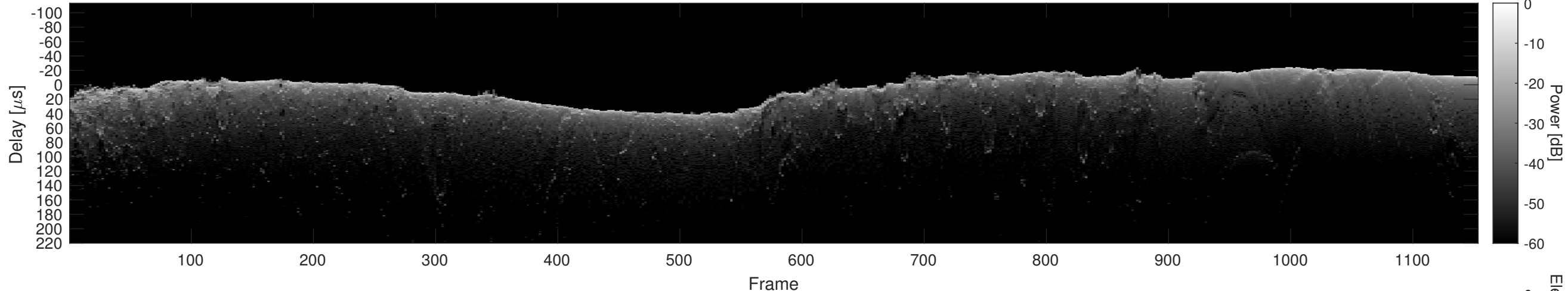
Orbit 11064, Cluttergram
