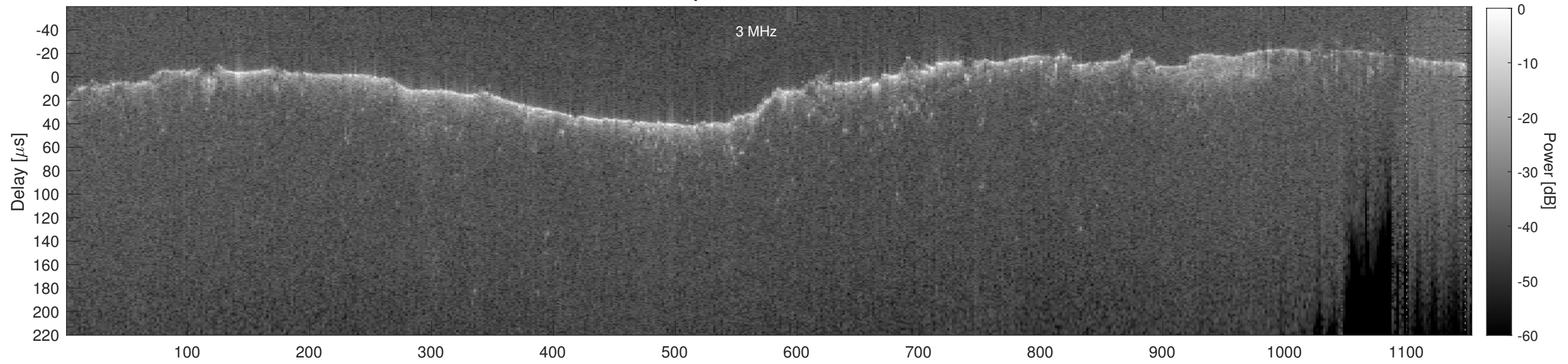
Orbit 11064, Cluttergram
