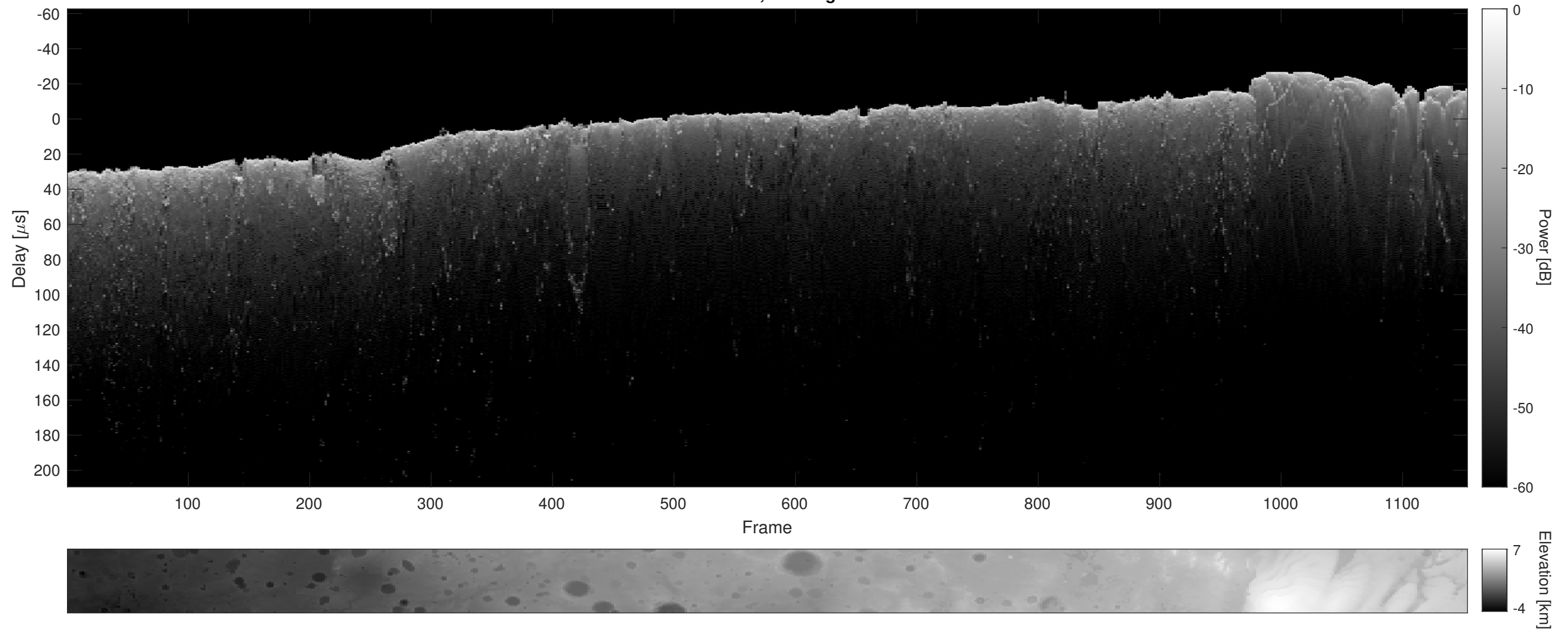
Orbit 11065, Cluttergram
