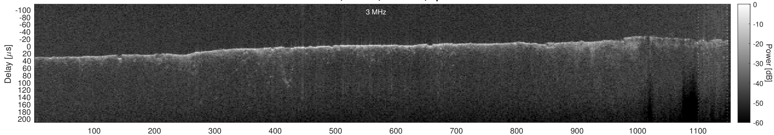
Orbit 11065, Cluttergram
