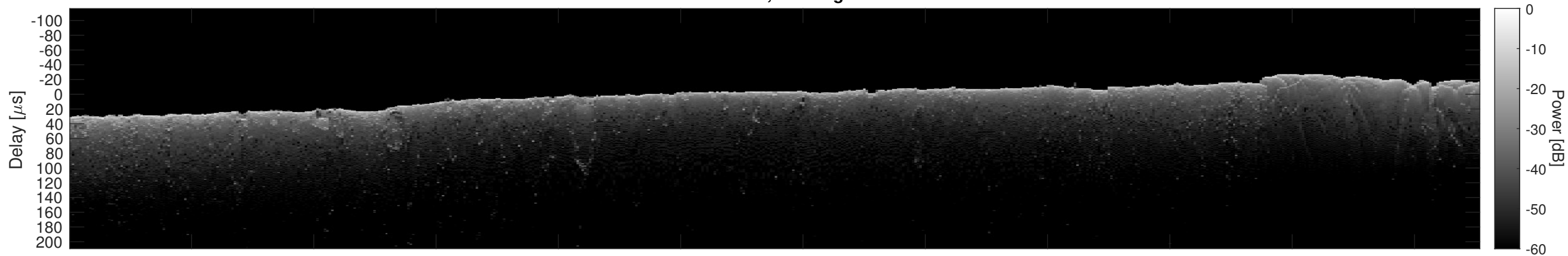
Orbit 11065, Cluttergram
