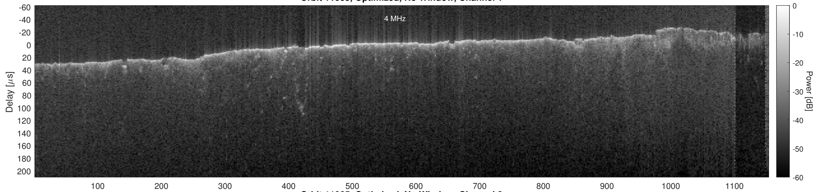
Orbit 11065, Optimized, No Window, Channel 2
