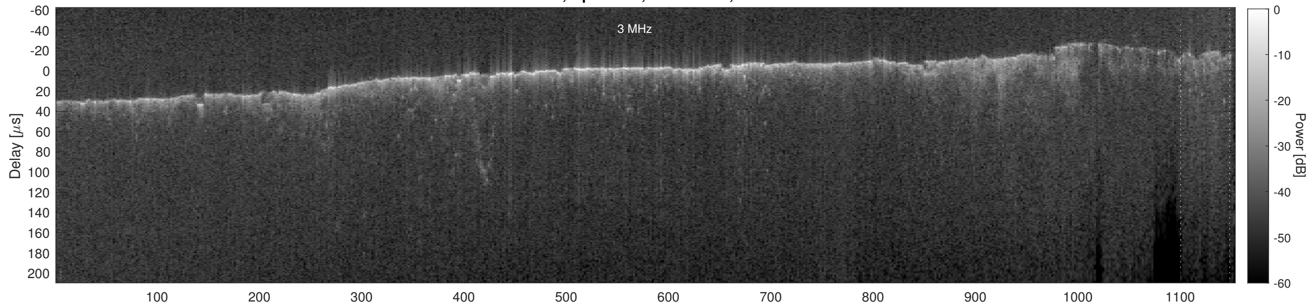
Orbit 11065, Cluttergram
