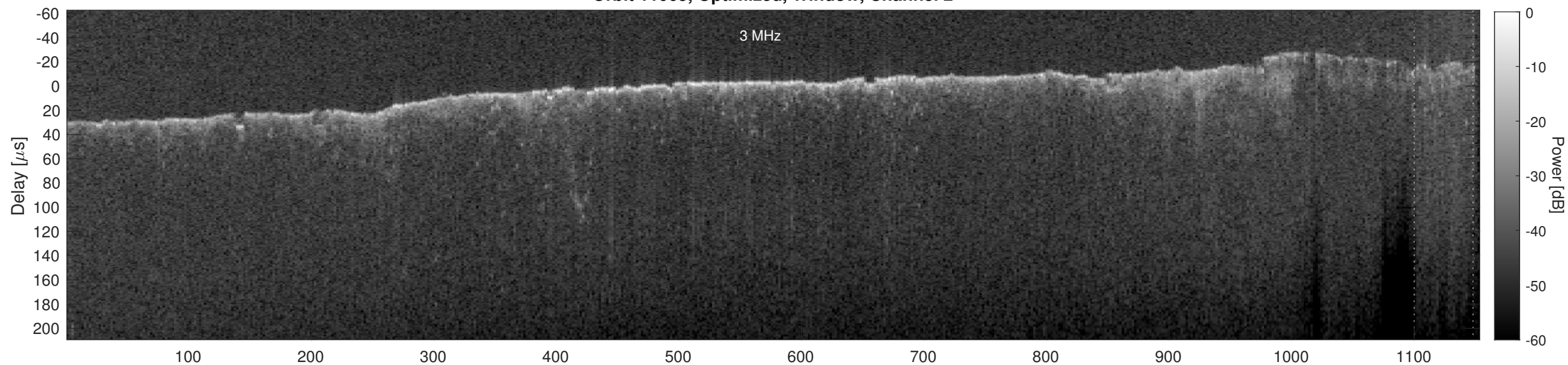
Orbit 11065, Cluttergram
